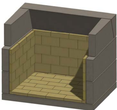
Figure 17. Sidewall Firebrick
