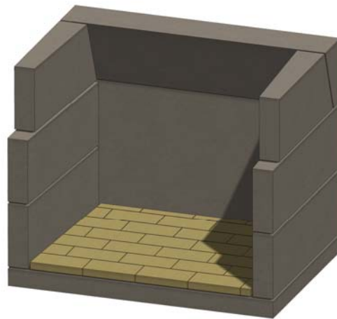
Figure 15. Floor Firebrick
